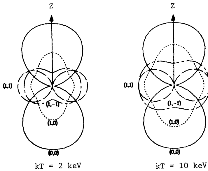
Fig. 3. Relative shapes of the four independent reaction rates \langle \sigma_{m,n} \rangle(\hat{v}') for the D(d,p) [top] and D(d,n) [bottom] reactions, at temperatures kT = 2 and 10 \text{ keV} . The polar angle is that between \hat{v}' and the Z-axis.
